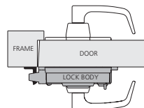
#3 STRIKE (Single or double door in-swing surface) PRODUCT NO. 2890-603
